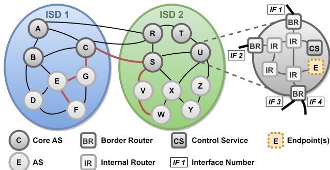
Figure 1: SCION topology example. Assuming the existence of three path segments C-G-E-F, C-S, and S-V-W, these three path segments can be combined into an end-to-end path from a host in AS F to a destination host in AS W.
