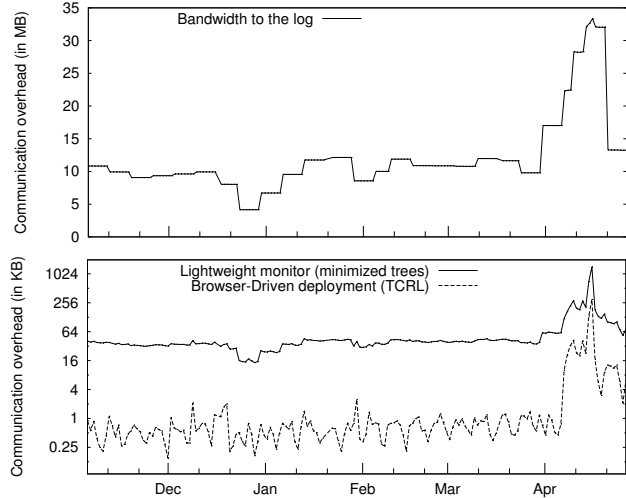
Figure 10. Bandwidth required by the log to receive certificate registrations and revocations (top chart), and by the browser to receive daily updates (bottom chart, note that the y-axis is in logarithmic scale).
