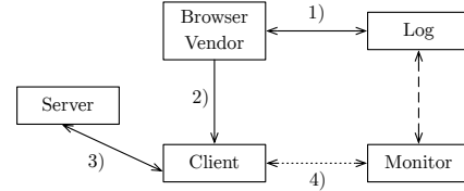
Figure 7. Browser-driven deployment model. Dotted and dashed lines represent optional and periodic communications, respectively.
